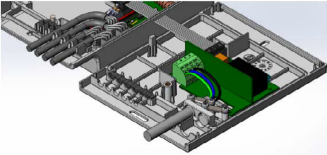
Figure 2: Installing cables to the 230 V meter unit EVH-R230
