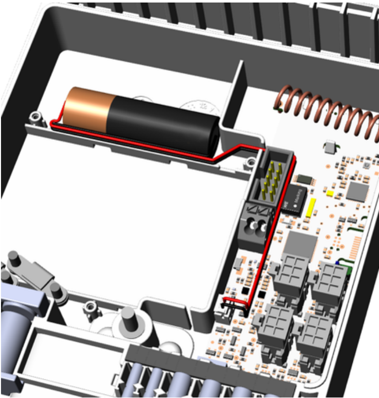
Figure 3: EVH-R230, connecting the backup battery
