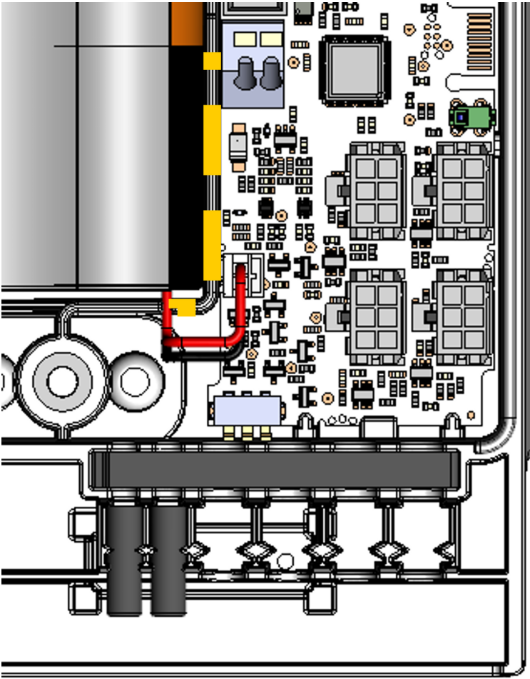
Figure 4: EVH-RB, connecting the battery pack
